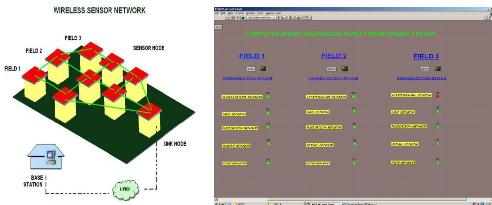
Figure 2: Wireless sensor Networks (WSN) Figure 3: Virtual Control using Lab VIEW
