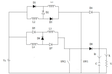
Figure 2.2 Mode 1 operation
