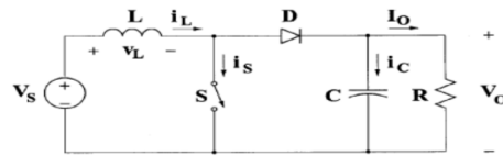
Figure 1.1 Boost Converter
