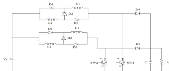
Figure 2.1 Interleaved Voltage Lift Boost Converter
