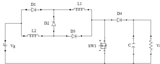
Figure 1.4 Switched Inductor Boost Converter
