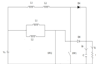
Figure 2.3 Mode 2 operation
