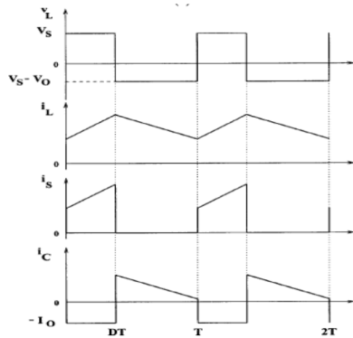
Figure 1.2 Waveforms of Boost Converter
