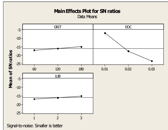
Fig.1 Effect of process parameters on Ra
