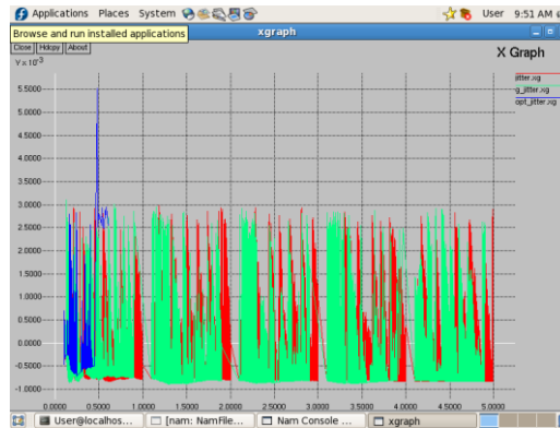
Fig.4 Comparison between jitter for Normal protocol, Only STR Protocol and STR Protocol +Cluster Head (LEACH)
