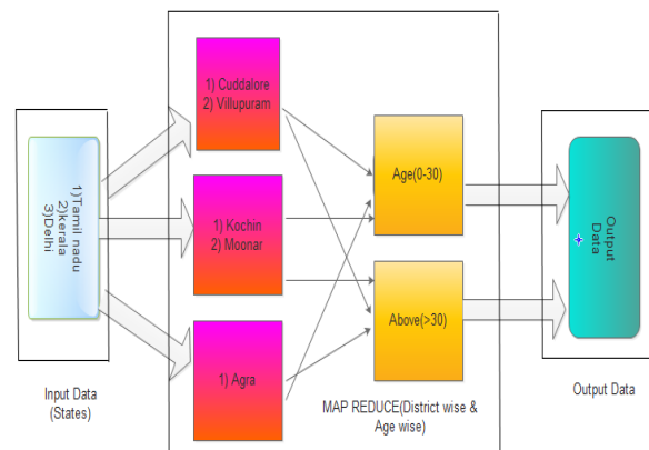
Figure 5 Map Reduce
