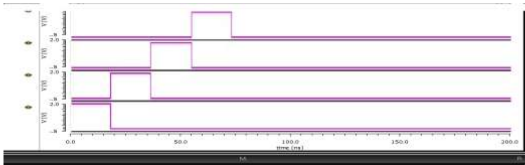
Fig 11: The Q-decoder outputs waveforms.
