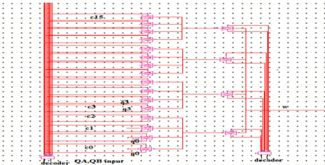
Fig 5: Quaternary 16-1 mux
