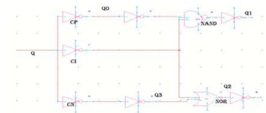
Fig 6: The Q-decoder logic structure.
