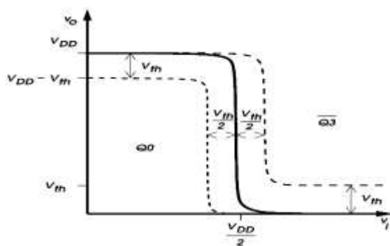
Fig 8: CP and CN transfer functions.
