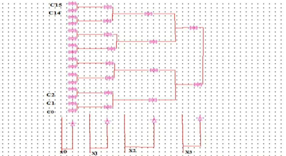
Fig 4: Binary 16-1 mux
